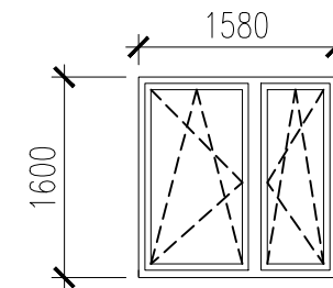
1x 1580x1600, plast
