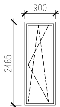
1x 900x2465, plast
